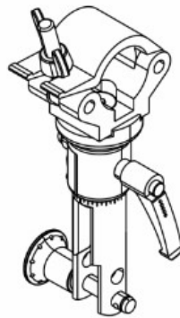
Image 20: VARIO CLAMP / General truss clamp for AiRAY, ViRAY, N-RAY, TiRAY, APS, N-APS frames and extension bar
