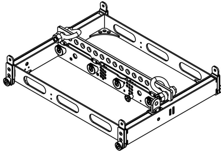
(Picture #14 FR-AR-Set / Frame for flying or ground stacking AiRAY / ViRAY or SC2-F / SCV-F in various combinations)
