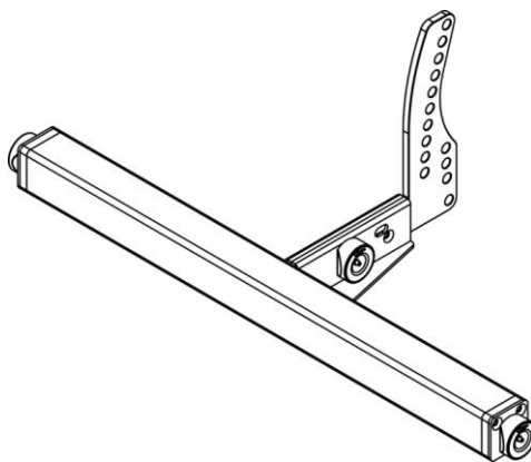
(Picture #18 AGA / AiRAY Ground Stack Adapter. Max 6x AiRAY cabinets can be stacked on SC2-F / SCV-F)
