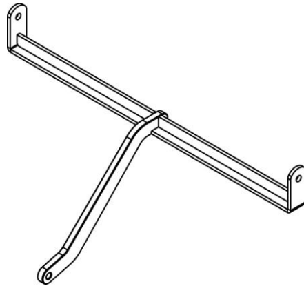
(Picture #19 AR-LINK / Adapter allows Top - Sub combination without additional frame)
